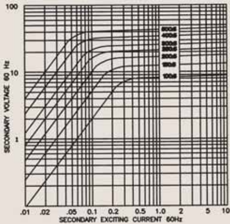
EXCITATION CURVE
