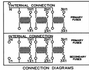
CONNECTION DIAGRAMS
