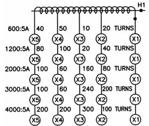
CONNECTION DIAGRAM
