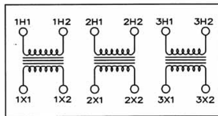
CONNECTION DIAGRAM
