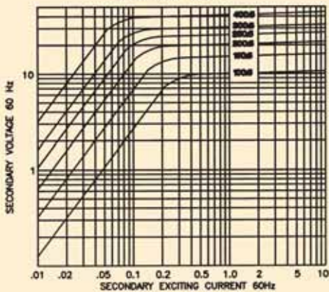
EXCITATION CURVE
